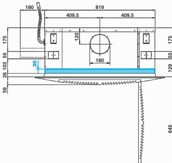
Models 4-5-6 (800x800)
