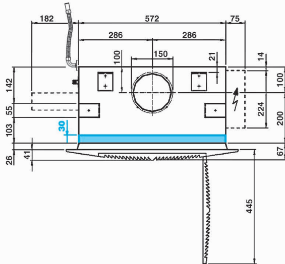
Models 0-1-2-3 (600x600)
