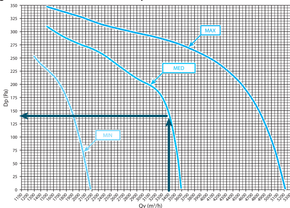
Diagram for Maestro MTL 64 "Available pressure"
