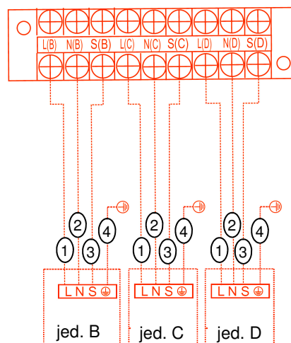
Svorkovnica HND 2015: modely 009-012
