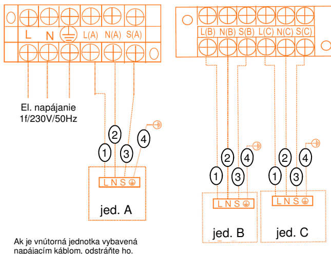
Svorkovnica HND 2015: modely 009-012
